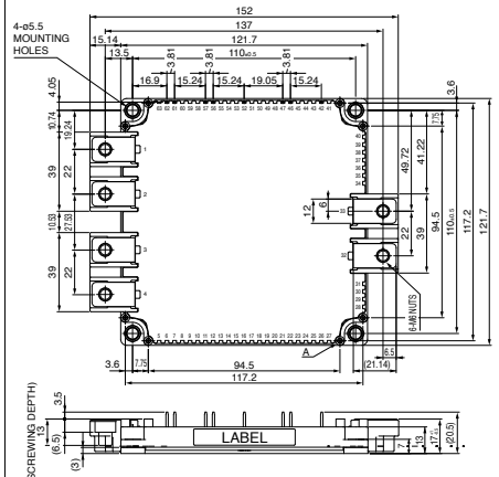
09 CM200TL/RL-12NF CM150,200TL/RL-24NF
