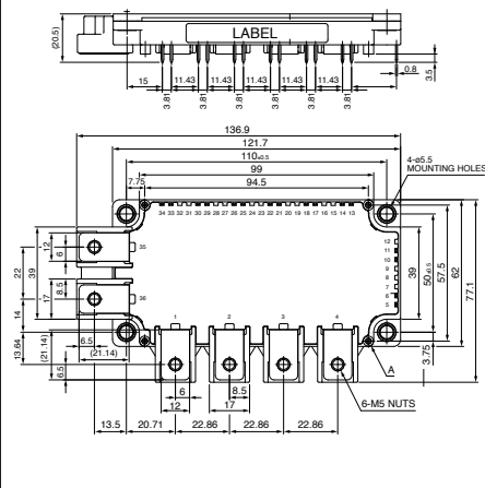
05 CM75TX-24S
