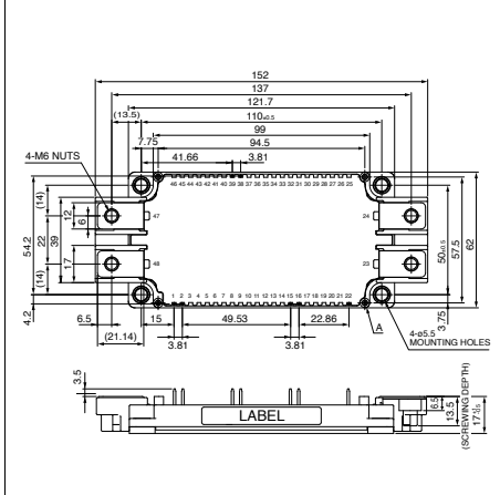
06 CM600,1000DXL-24S
