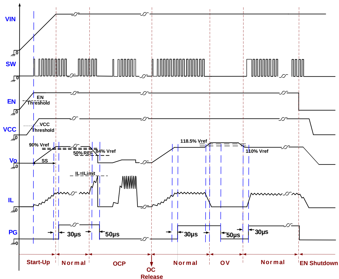
Figure 2: Time Sequence
